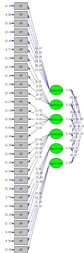
Chi-Square=854.73, df=362, P-value=0.00000, RMSEA=0.01
